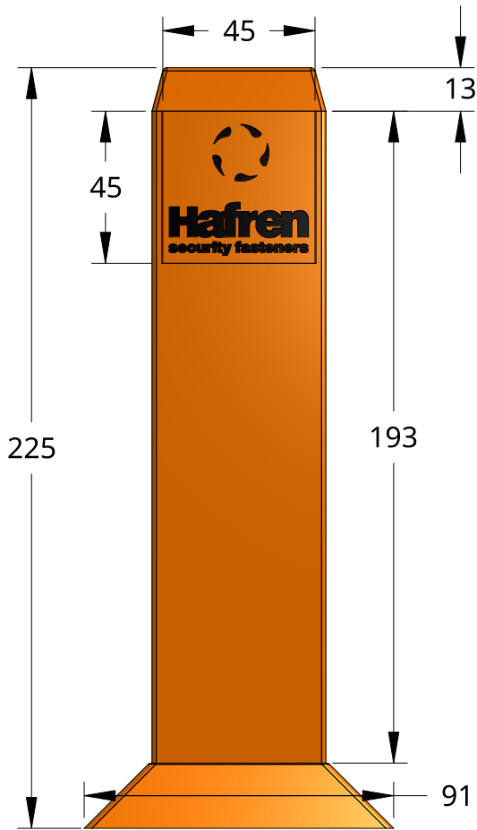
Front SCALE 1:2
