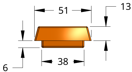
Front SCALE 1:2
