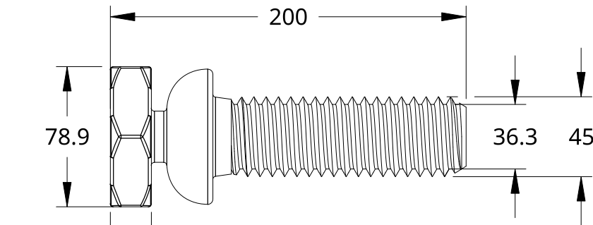
Front SCALE 1:3
